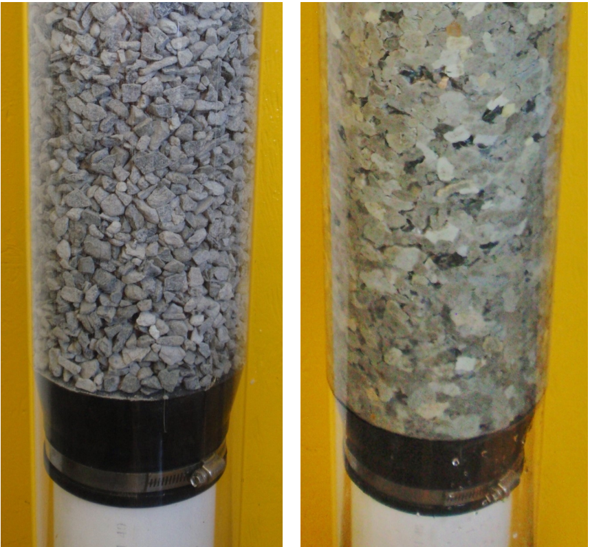
Chip bentonite before (left) and after (right) initial hydration. The chip bentonite surrounds a white PVC casing positioned inside a clear plastic pipe (for demonstration purposes). The chips are supported by a shale trap [see Figure 5, page 22].
